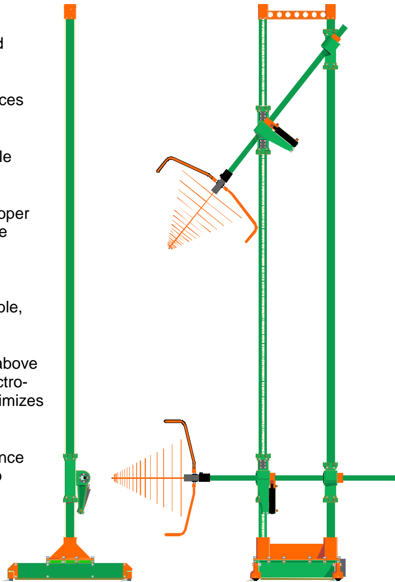
Depicted with top antenna focal point in extreme elevation, sighted at zero EUT height, and 3-meter EUT distance.
