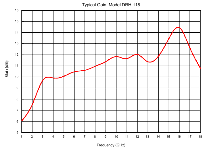
Model DRH-118
